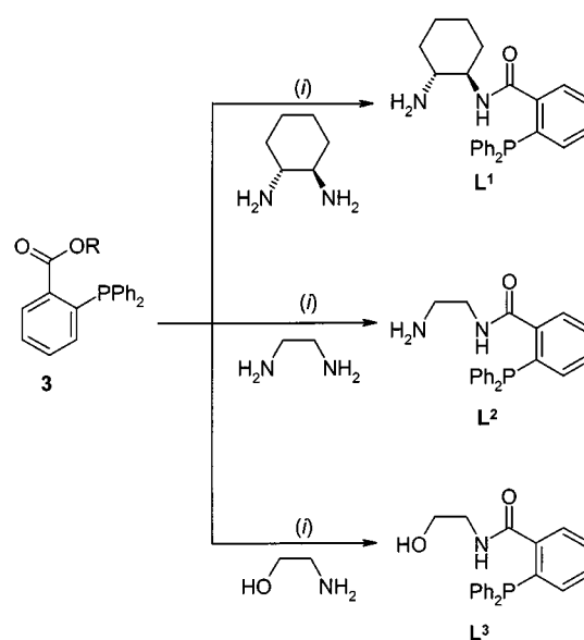
Scheme 1. Synthesis of the Ligands L 1 , L 2 , and L 3 ; R = N -succinimido; (i) dichloromethane, room temperature
