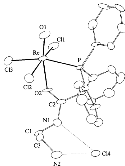
Figure 2. ORTEP drawing of complex 5 with the atom numbering scheme; thermal ellipsoids are drawn at the 30% probability level
