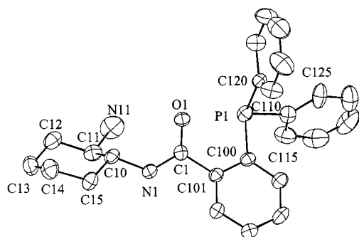
Figure 1. ORTEP drawing of ligand L 1 with the atom numbering scheme; thermal ellipsoids are drawn at the 30% probability level; selected mean bond lengths [Å] and angles [°]: C(1)–O(1) 1.231(8), N(1)–C(1) 1.329(9), N(1)–C(10) 1.448(9), C(11)–N(11) 1.449(11), C(1)–C(101) 1.498(10), P(1)–C(100) 1.848(8), P(1)–C(110) 1.838(9), P(1)–C(120) 1.837(8), av. (C–C) cyclohex 1.51(1), av. (C–C) phenyl 1.37(2); N(1)–C(1)–O(1) 123.3(7), O(1)–C(1)–C(101) 120.7(7), N(1)–C(1)–C(101) 116.1(7), C(10)–N(1)–C(1) 124.5(6)
