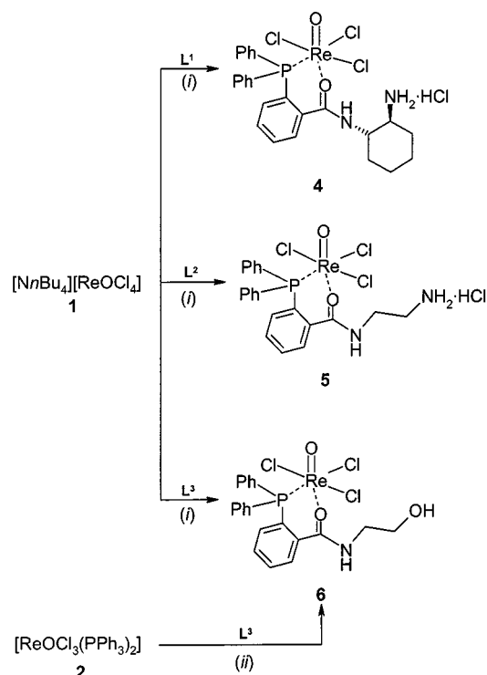
Scheme 2. Synthesis of the complexes 4–6 ; (i) MeOH, room temperature; (ii) dichloromethane, room temperature
