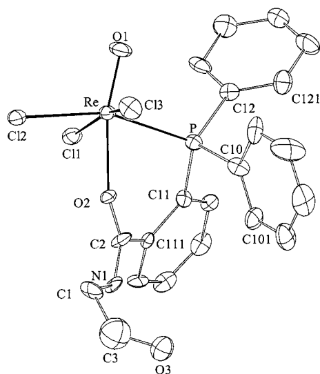
Figure 3. ORTEP drawing of complex 6 with the atom numbering scheme; thermal ellipsoids are drawn at the 30% probability level; selected mean bond lengths [Å] and angles [°]: Re–O(1) 1.659(10), Re–O(2) 2.133(10), Re–Cl(1) 2.367(5), Re–Cl(2) 2.377(4), Re–Cl(3) 2.355(4), Re–P 2.425(5), C(2)–O(2) 1.26(2), N(1)–C(2) 1.28(2), N(1)–C(1) 1.46(2), av. P–C 1.82(2); O(1)–Re–O(2) 167.2(5), O(1)–Re–Cl(1) 97.6(4), O(1)–Re–Cl(2) 107.5(4), O(1)–Re–Cl(3) 95.5(4), O(1)–Re–P 93.1(4), Cl(1)–Re–Cl(3) 166.1(2), Cl(2)–Re–Cl(3) 85.9(2), Cl(1)–Re–P 89.0(2), Cl(2)–Re–P 159.3(2), O(2)–Re–Cl(1) 85.3(4), Cl(3)–Re–P 94.9(2), Re–O(2)–C(2) 141.0(13), O(2)–C(2)–N(1) 121(2), O(2)–Re–P 74.5(3), C(2)–N(1)–C(1) 124.1(14), N(1)–C(2)–C(11) 118(2)
